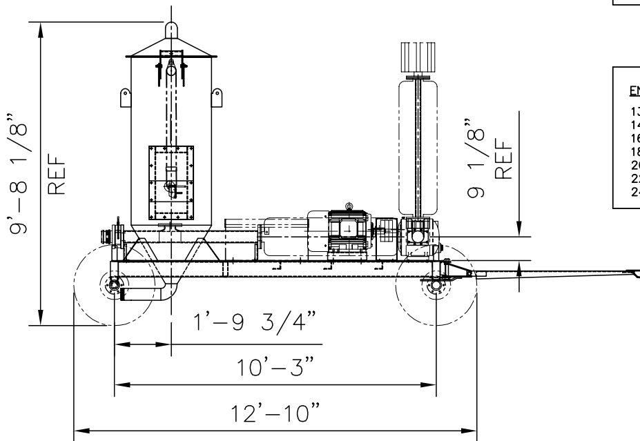
ELEVATION VIEW SCALE: 1/4"=1'-0"
